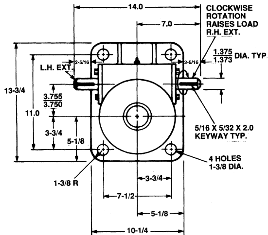
3" Diameter x .660 Lead Lifting Screws
