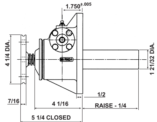
Upright: M-7002
