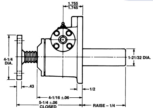
Upright: M-9002
