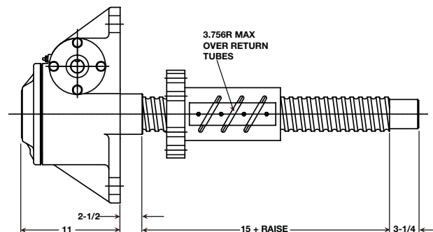
Inverted Rotating: DM-2861
