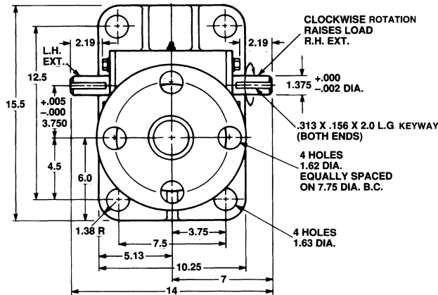
3 \frac{3}{4} " Diameter x .666 Lead Lifting Screws
