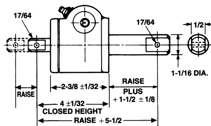
Double Clevis: CCM-2625
