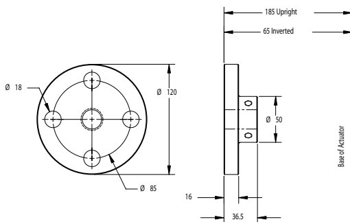
Top Plate G9005-6
