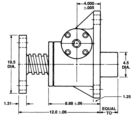
Upright: M-9035
