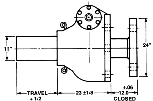
Inverted: M-2249
