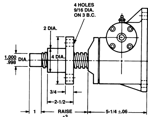
Inverted: M-9004
