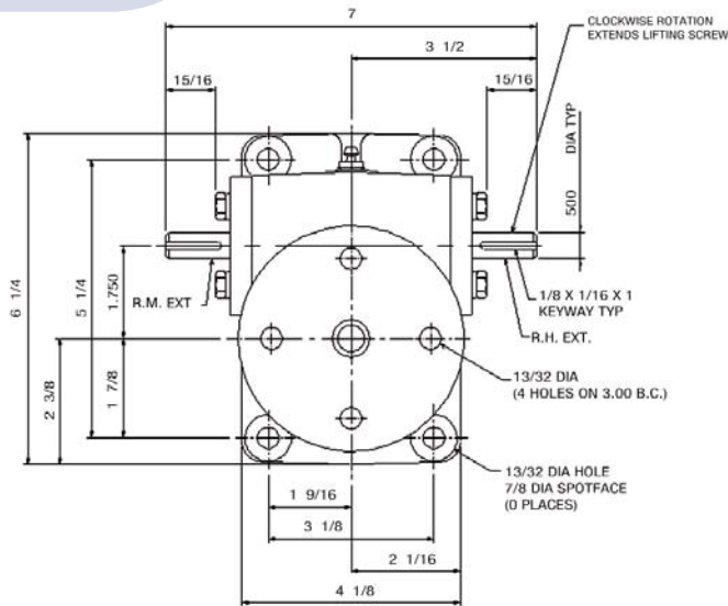
1" DIAMETER X .250 LEAD LIFTING SCREW
