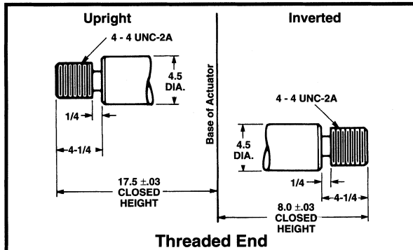
4 1/2" Diameter x .666 Lead Lifting Screws
