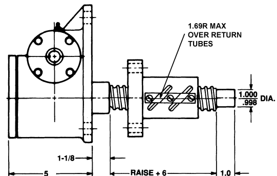
Inverted Rotating: DM-9811
