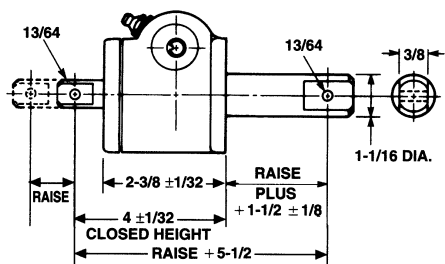
Double Clevis: CCM-2555
