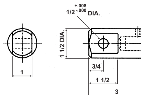
Clevis End (Optional) SK2800-4-2A
