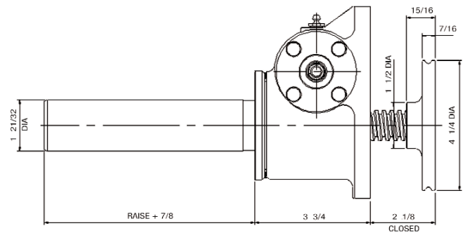
Inverted: M-90002
