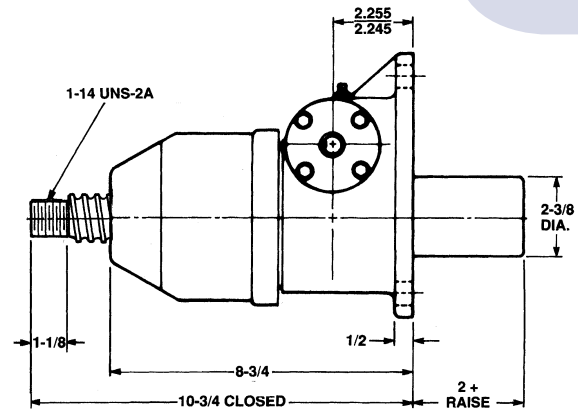
Upright: M-9805
