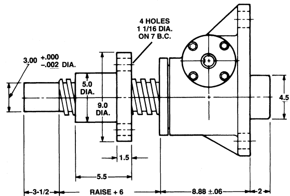
Upright Rotating: UM-9036
