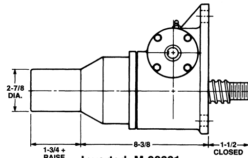
Inverted: M-98091
