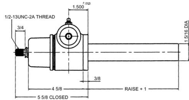
Upright: M-28750
