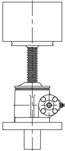
One end fixed, one end free
