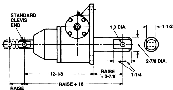
Double Clevis
