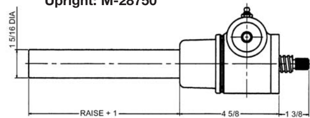
Inverted: M-28749
