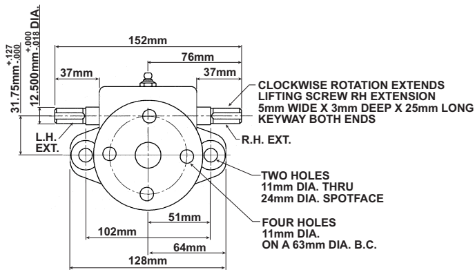
Top View: MET-2501
