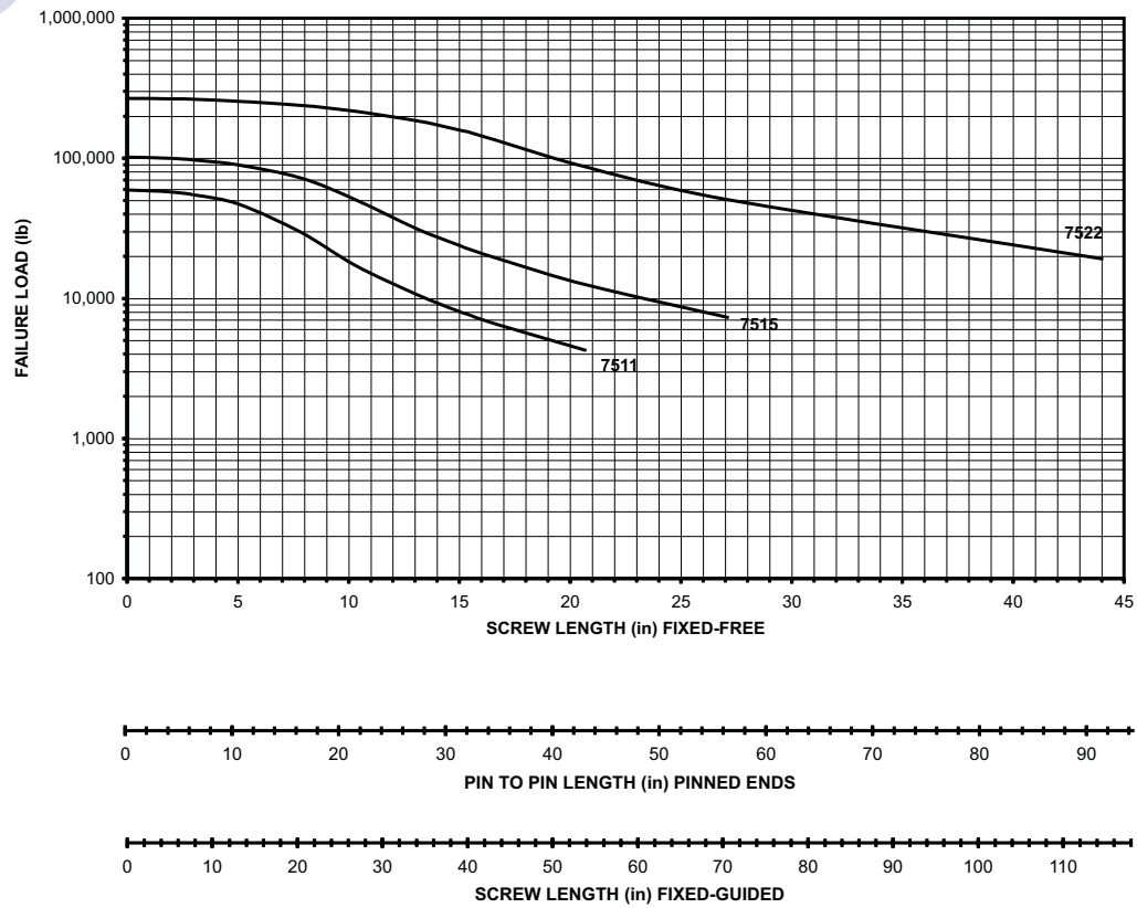
Screw Column Strength Chart For Continuous Duty Cycle Actuators
