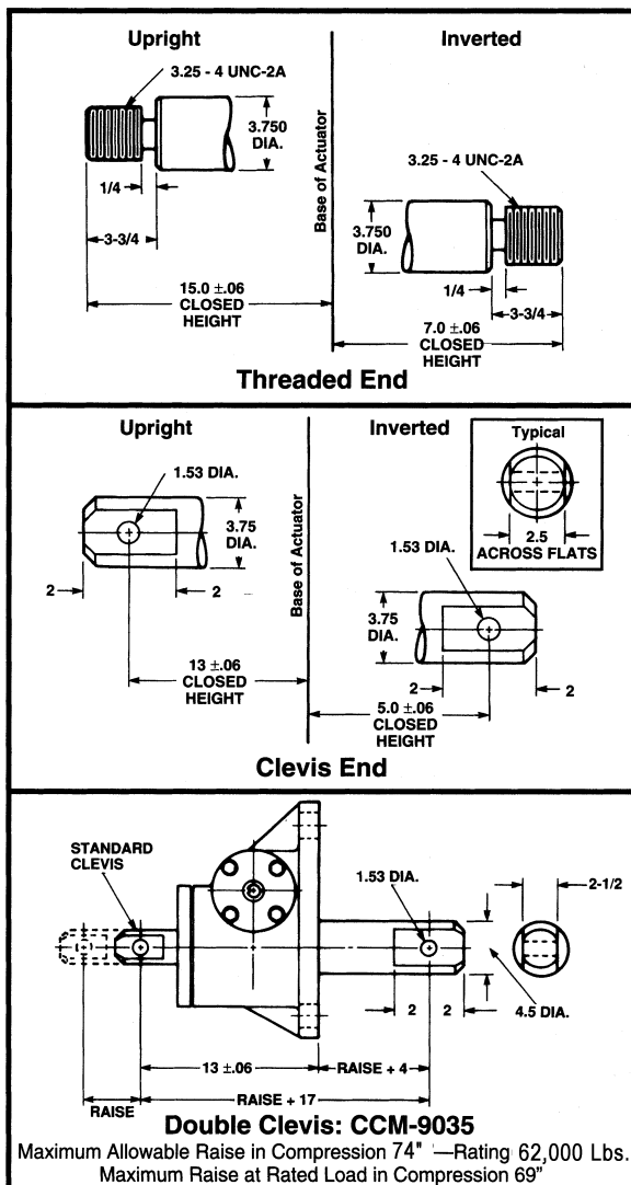
3 \frac{3}{4} " Diameter x .666 Lead Lifting Screws
