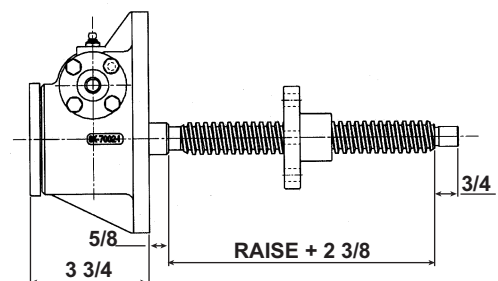
Inverted Rotating: DM-7003
