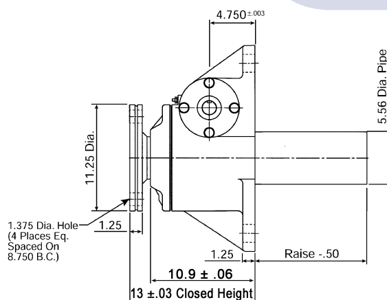
Upright: M-9050
