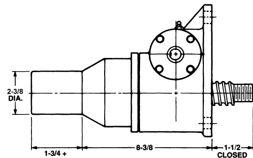
Inverted: M-9809
