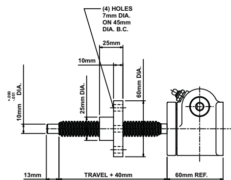
Upright Rotating: MET-UM-2626
