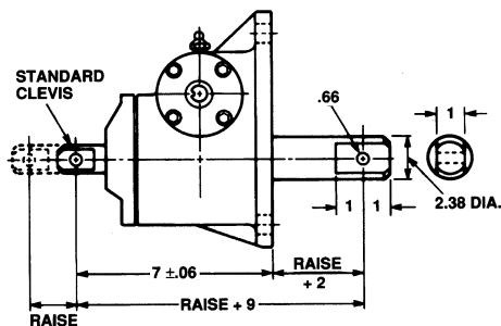
Maximum Allowable Raise in Compression 22" —Rating 6500 Lbs. Maximum Raise at Rated Load in Compression 17"
