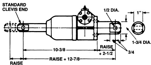
Double Clevis
