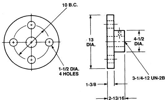
Top Plate (Optional) SK2800-1-60A
