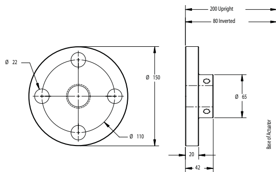
Threaded End G9010-6
