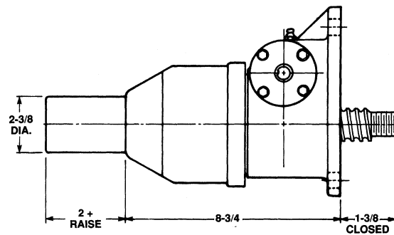
Inverted: M-9805
