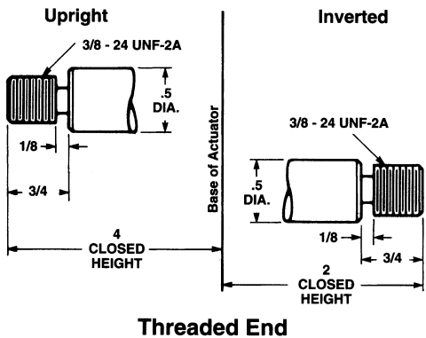
Threaded End
