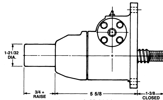
Inverted: M-9801
