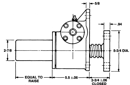
Inverted: M-9014
