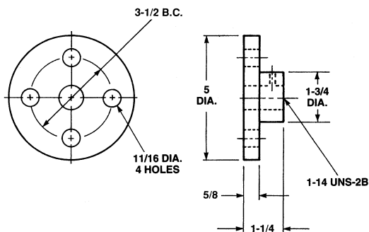
Top Plate (Optional) SK2800-1-5A
