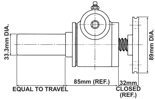
Inverted: MET-2500
