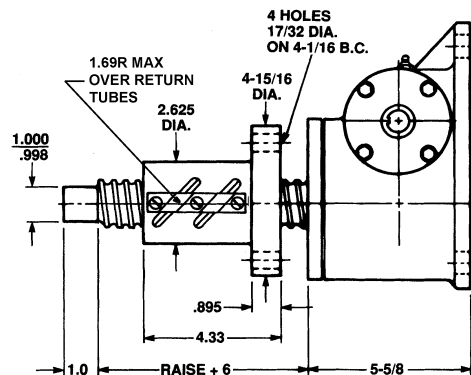
Upright Rotating: UM-9811
