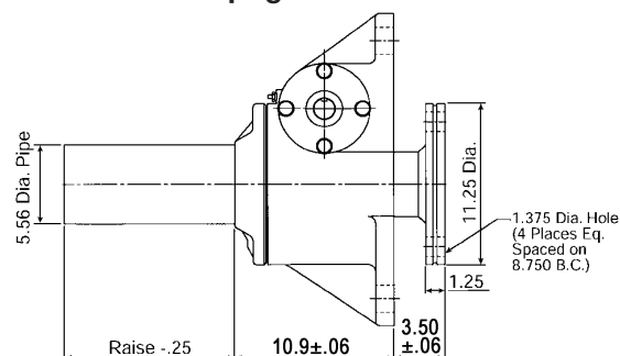
Upright: M-9050
