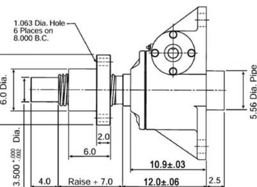
Upright Rotating: UM-9051
