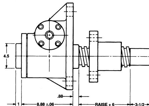
Inverted Rotating: DM-9036
