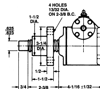
Upright Rotating: UM-1803
