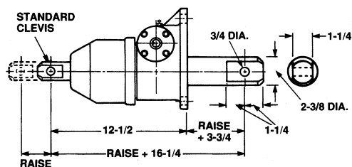
Double Clevis
