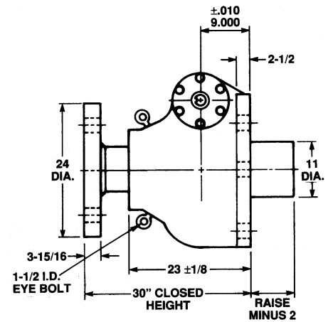
Upright: M-2250
