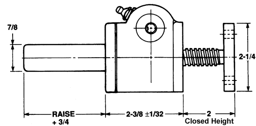
Inverted: M-2624
