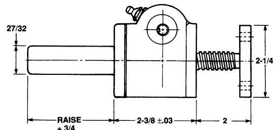
Inverted: M-2554
