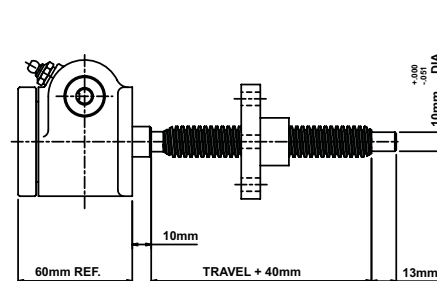
Inverted Rotating: MET-DM-2626
