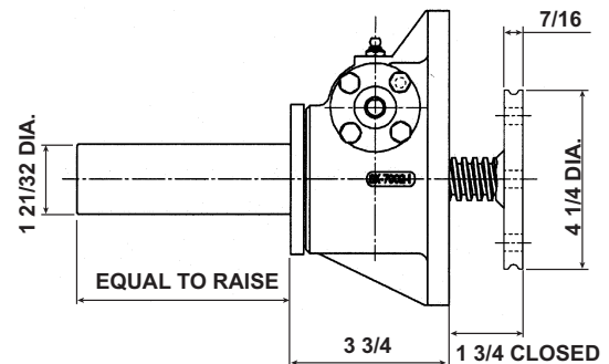
Inverted: M-7001
