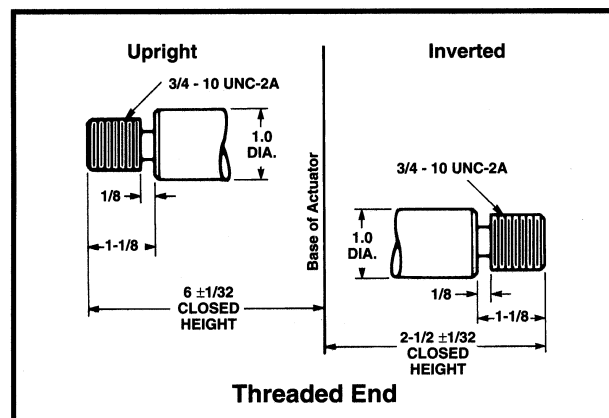
1" Diameter x .250 Lead Lifting Screws
