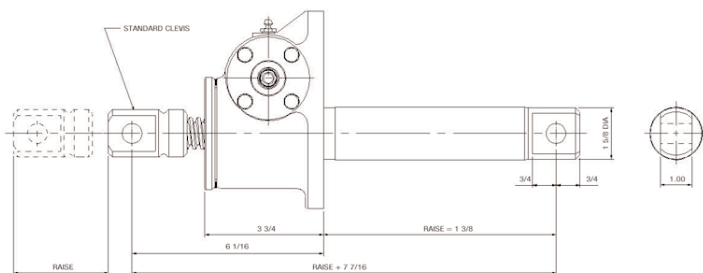
Double Clevis: CCM-90003
