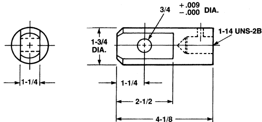
Clevis End (Optional) SK2800-4-5A
