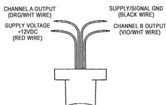
Electrical Connections
