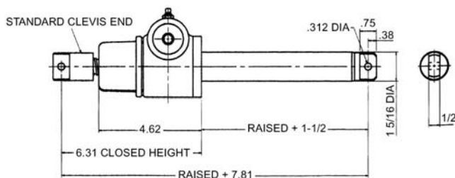
Double Clevis: CCM-28750
