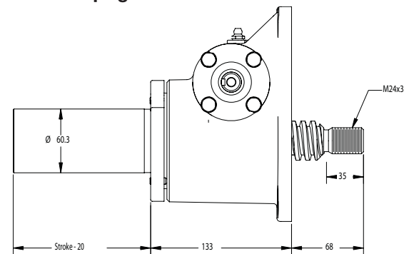
Inverted: G9004
