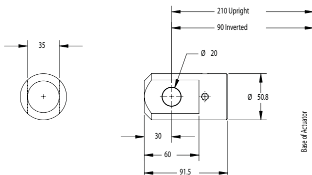
Clevis End G9005-11
