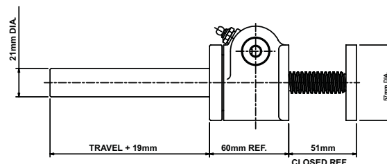
Inverted: MET-2624
