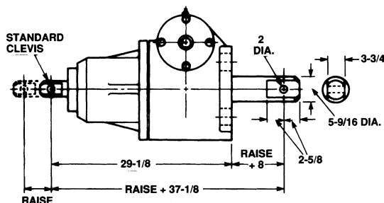
Double Clevis
