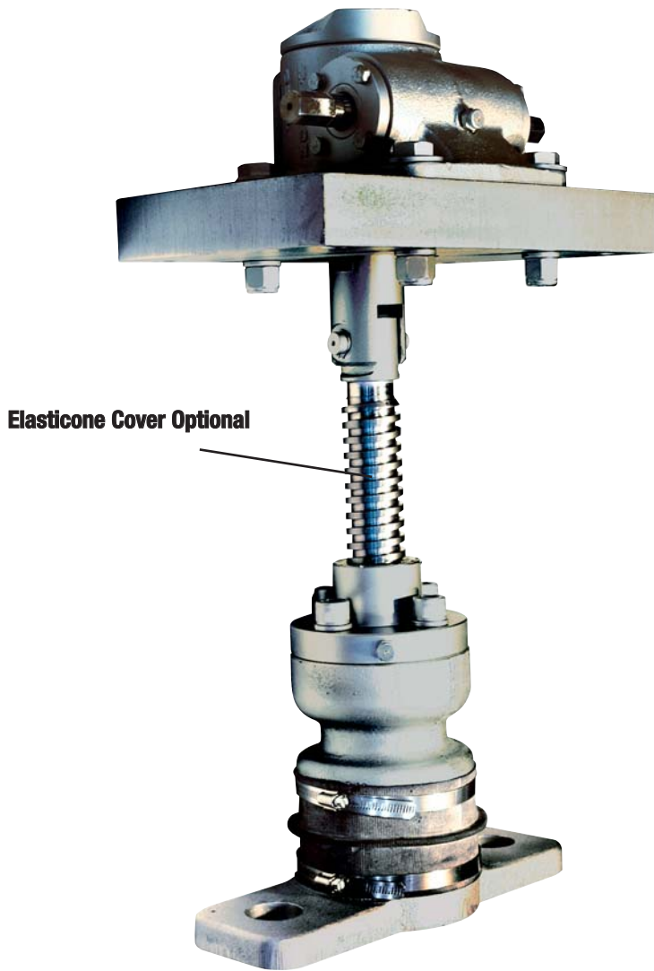
Inverted Rotating Style Anode Jack
