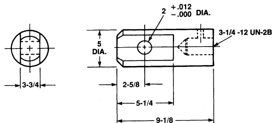
Clevis End (Optional) SK2800-4-60A
