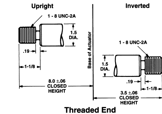
1 1/2" Diameter x .375 Lead Lifting Screws
