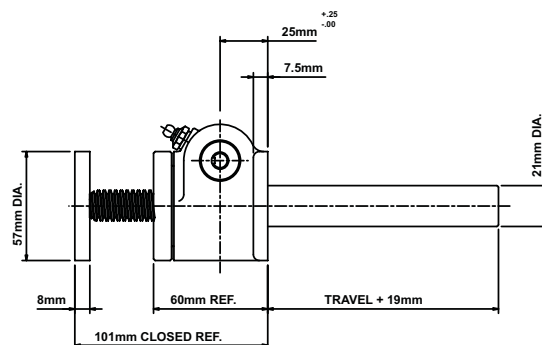
Upright: MET-2625
