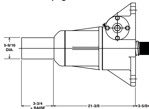
Inverted: M-9859
