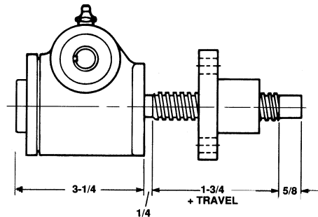
Inverted Rotating: DM-2502
