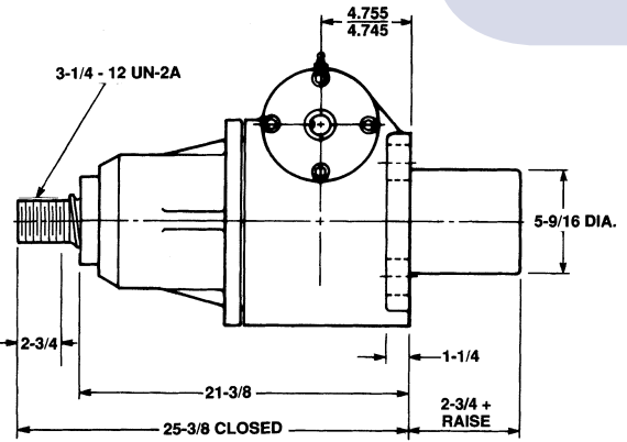
Upright: M-2860
