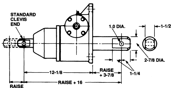
Double Clevis
