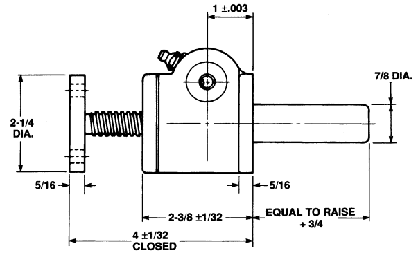
Upright: M-2625
