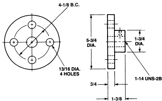
Top Plate (Optional) SK2800-1-10A
