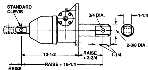
Double Clevis
