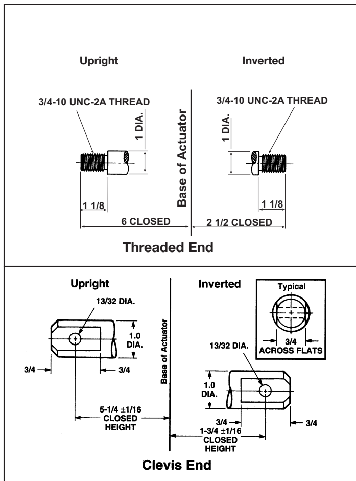
1" Diameter x .250 Lead Lifting Screw
