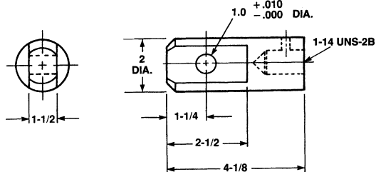
Clevis End (Optional) SK2800-4-10A
