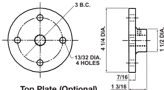
Top Plate (Optional) SK2800-1-2A
