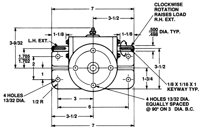
1" Diameter x .250 Lead Lifting Screws
