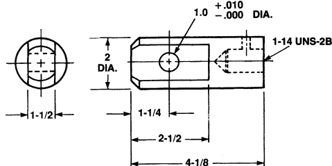
Clevis End (Optional) SK2800-4-10A
