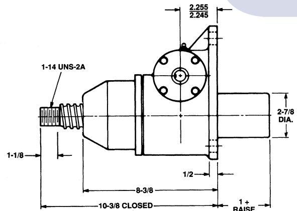
Upright: M-9810
