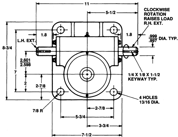
1 1/2" Diameter x 1.000 Lead Lifting Screws
